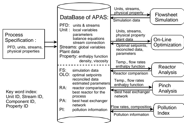
Fig. 2 Database Structure of Advanced Process Analysis System
