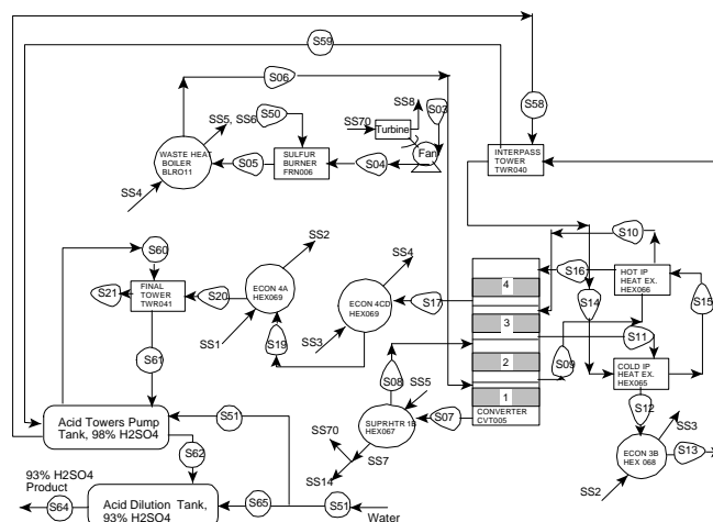
Fig. 3 Flowsheet Diagram for Contact Process
