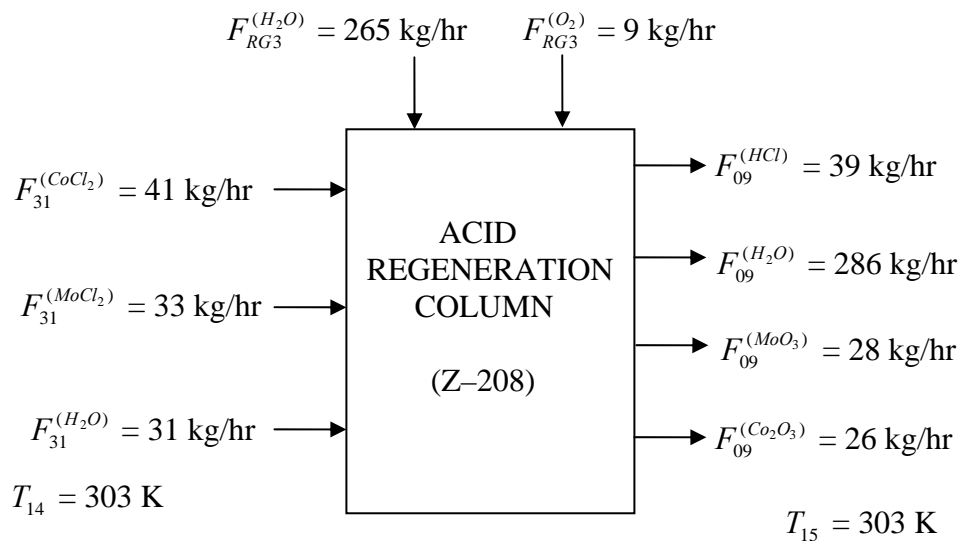
Figure C2.22. Input – Output Component Balance for Acid Regeneration Column (Z-208)
