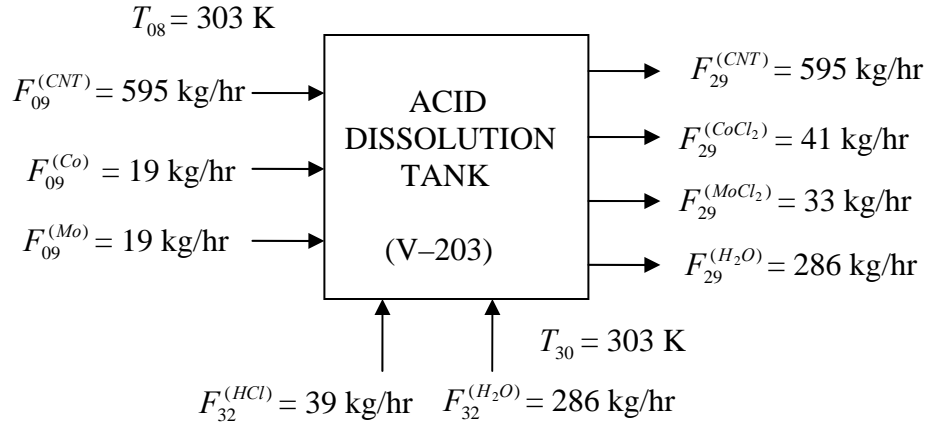
Figure C2.18. Input – Output Component Structure for Acid Dissolution Tank (V–203)
