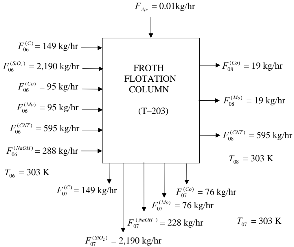
Figure 2.16. Input – Output Component Structure for Flotation Column (T-203)
