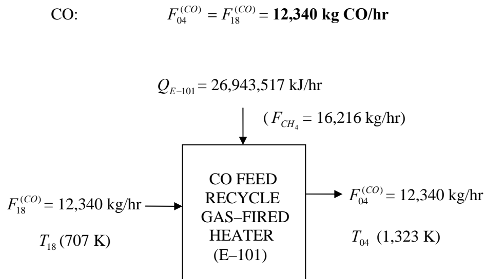
Figure C1.8. Input – Output Component Structure for Gas-Fired Heater (E-101)
