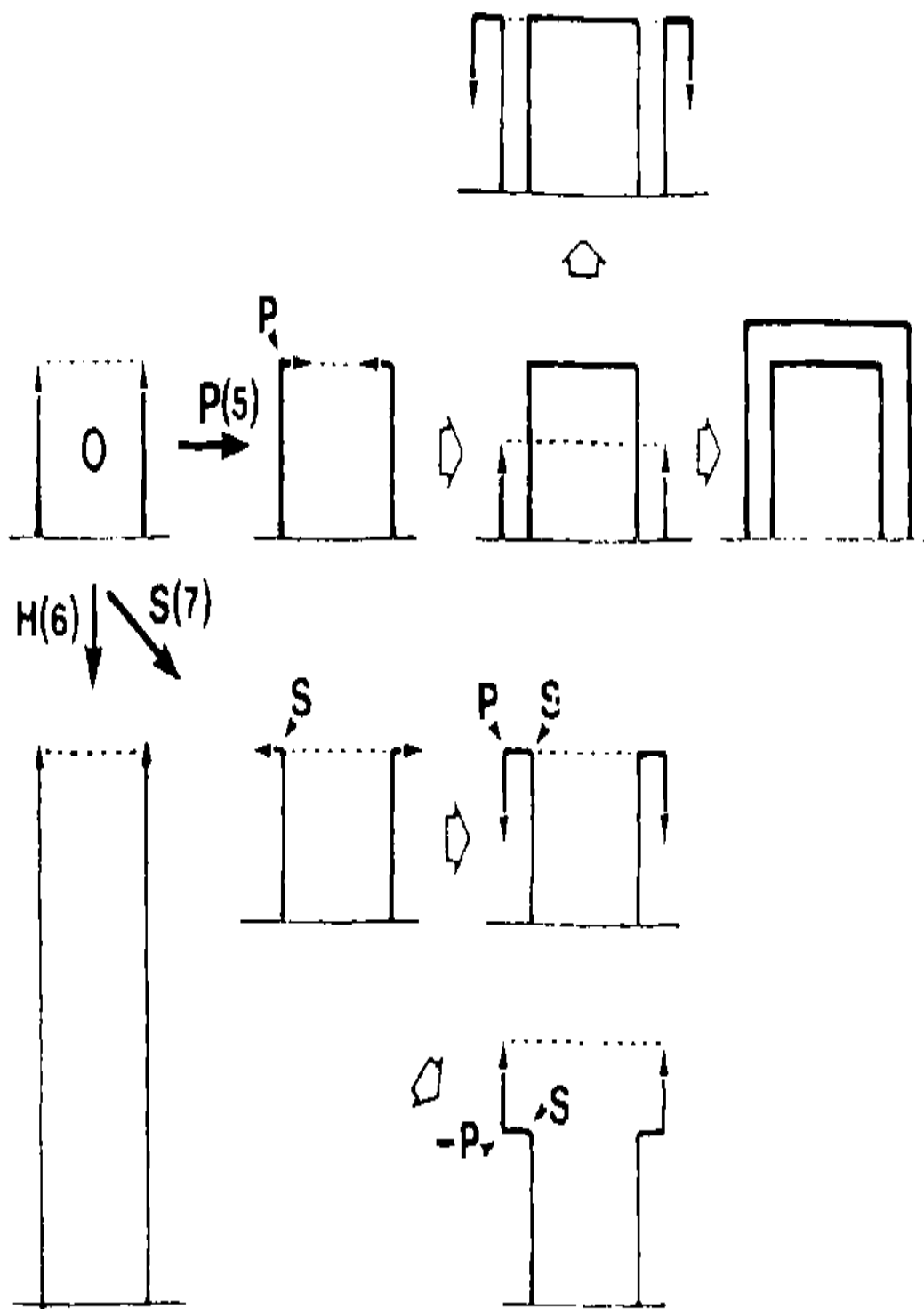
Figure 2.9. Schematic Depicting the Various Carbon Nanotube Growth Probabilities Starting from a Nucleus O by the Addition of Hexagons, H(6) , Pentagons, P(5) , and Heptagons, S(7) , successive addition of heptagons causes an opening up (Iijima et al, 1992).
