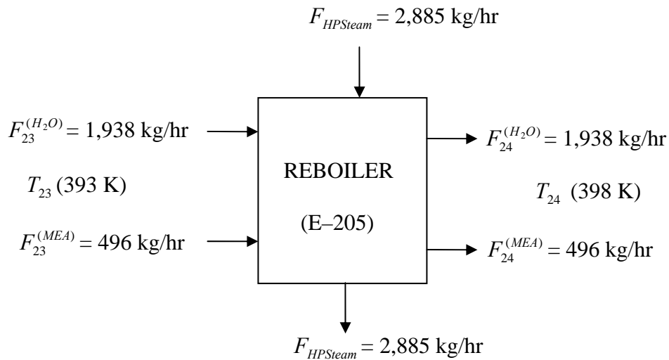
Figure C2.12. Input – Output Component Structure for Reboiler (E-205)
