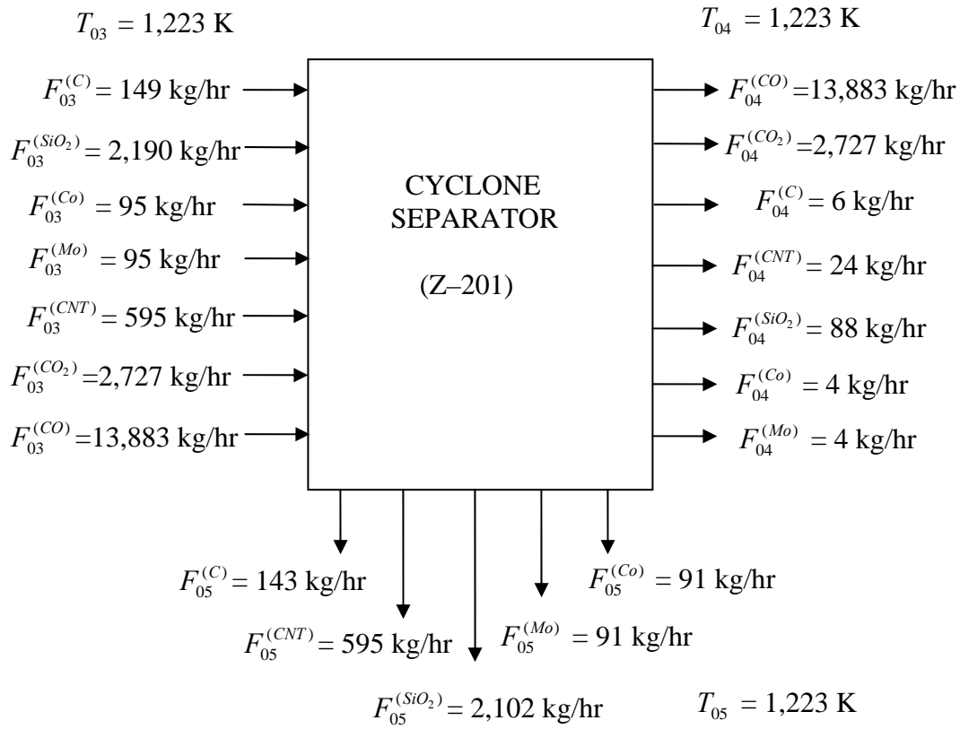
Figure C2.4. Input – Output Component Structure for Cyclone Separator (Z-201)
